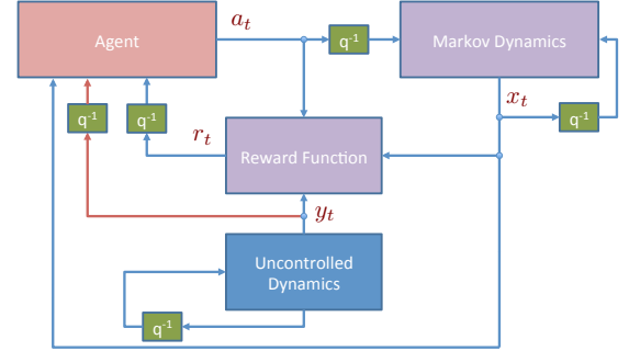
Fig. 1. The interaction between the learning agent and the environment. Here q^{-1} denotes a unit delay, that is, any information sent through such a box is received at the beginning of the next time step.
