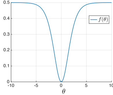
Figure 6. The image of f .
