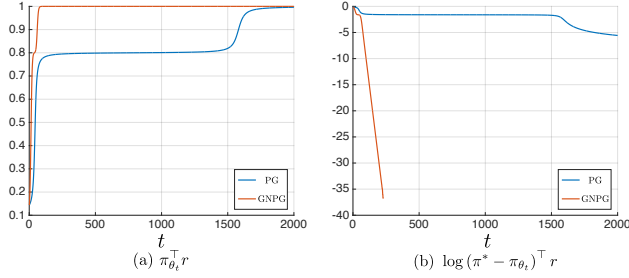
Figure 4. PG and GNPG on r = (1.0, 0.8, 0.1)^T .
