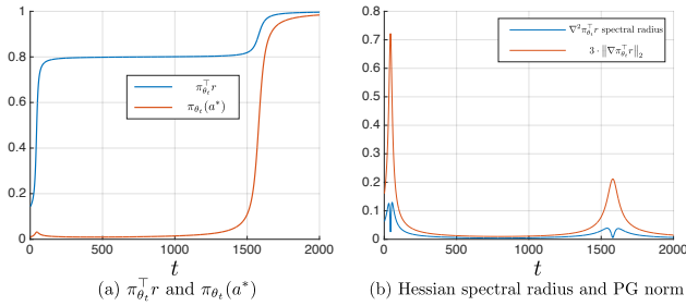
Figure 3. PG results on r = (1.0, 0.8, 0.1)^\top .
