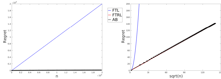
Figure 6: Experimental results for worst-case data.
