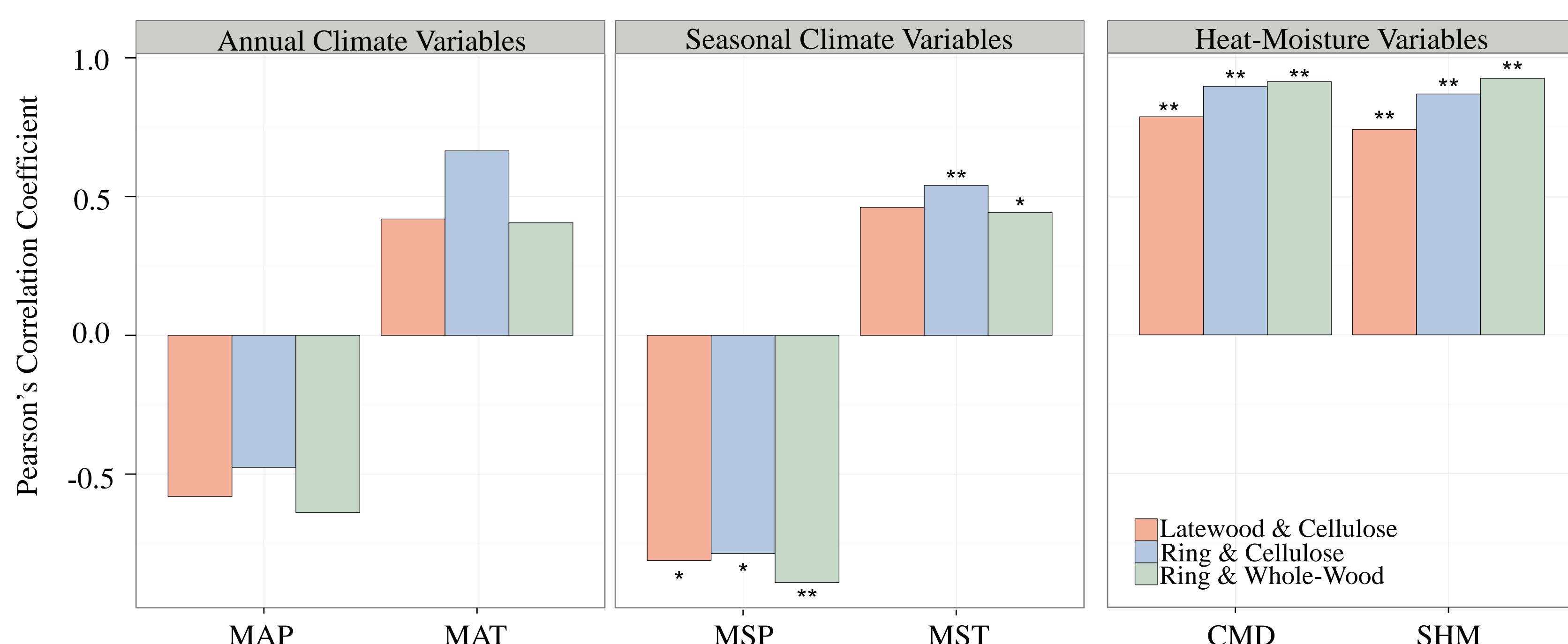
Fig 3. Correlations of ^{13}C/^{12}C to mean annual precipitation (MAP), mean annual temperature (MAT), mean summer precipitation (MSP), mean summer temperature (MST), climatic moisture deficit (CMD), summer heat:moisture (SHM).
