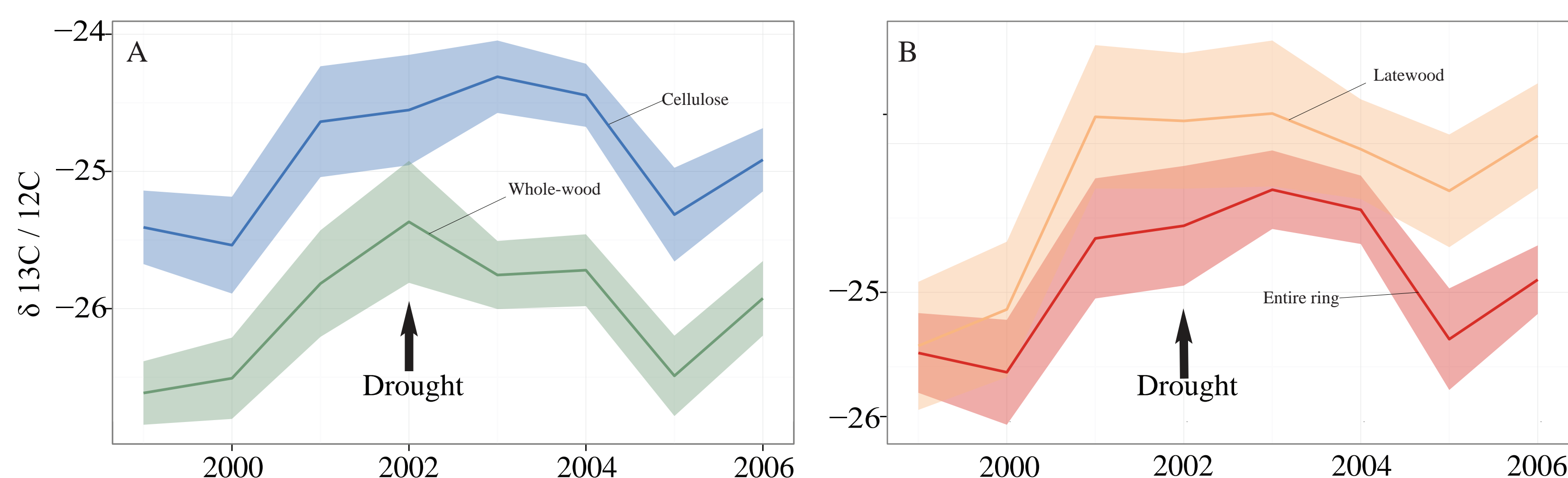
Fig 2. Ratio of Carbon 13 to Carbon 12 (deviations from Vienna Pee Dee Belemnite) by year. Cellulose (blue) and whole-wood (green) are compared on the left; latewood (orange) is compared to the entire ring (red) on the right.
