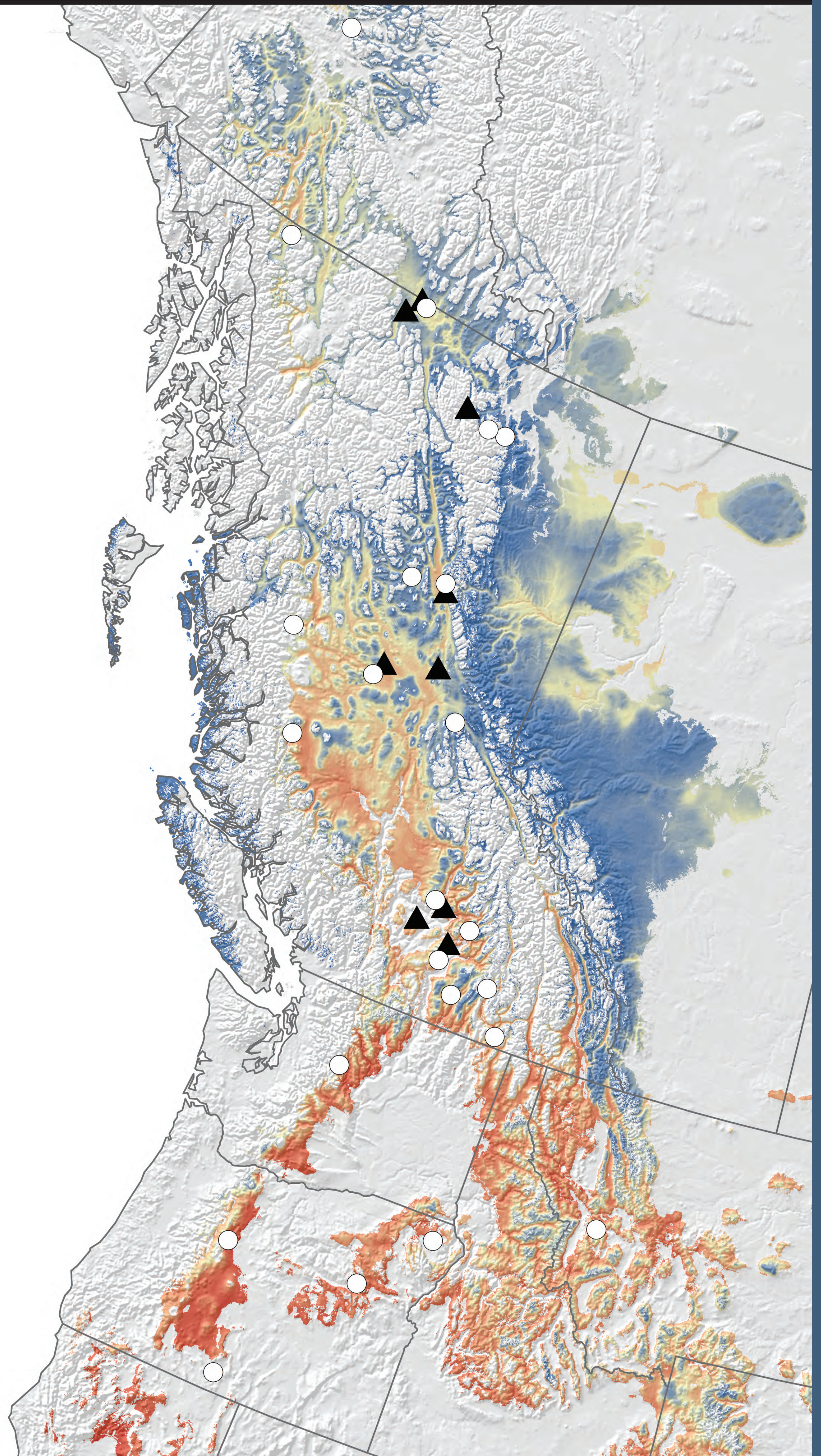
Fig 1. Lodgepole pine ( Pinus contorta ) species range in western North America coloured by Hargreaves Climatic Moisture Deficit (mm, 1961-1990). Circles indicate seed sources; triangles represent planting sites.
